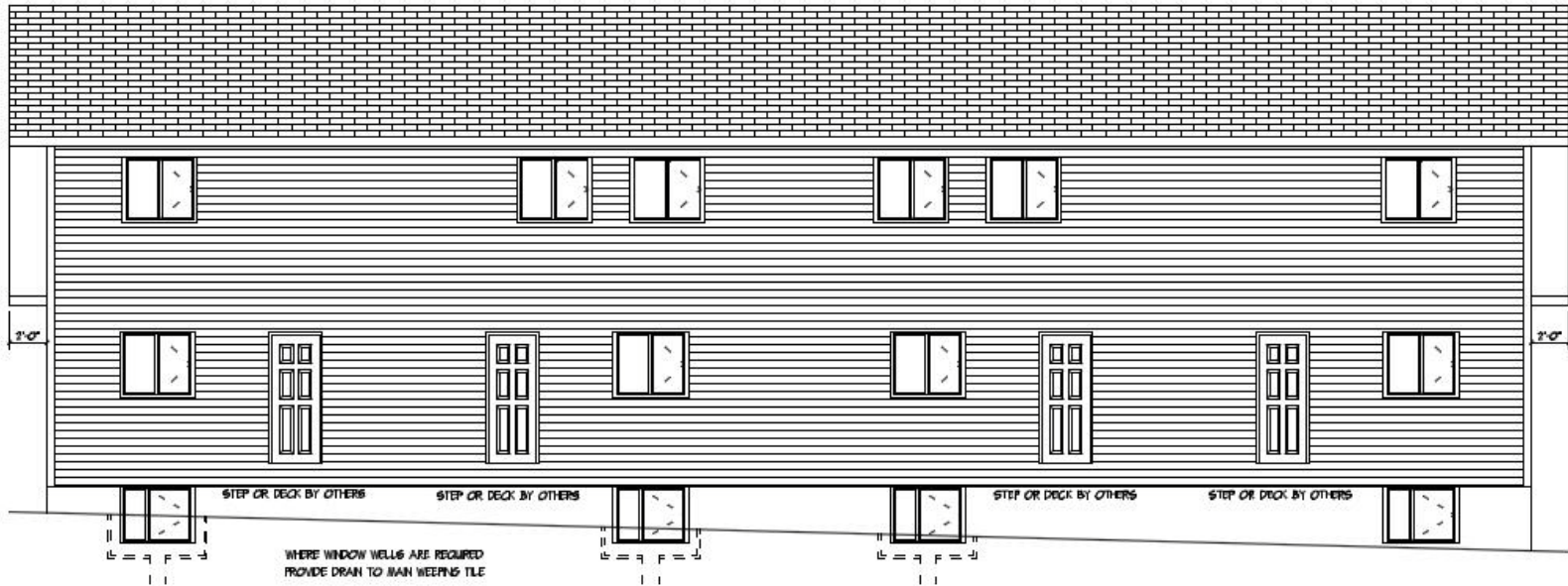
REAR ELEVATION
