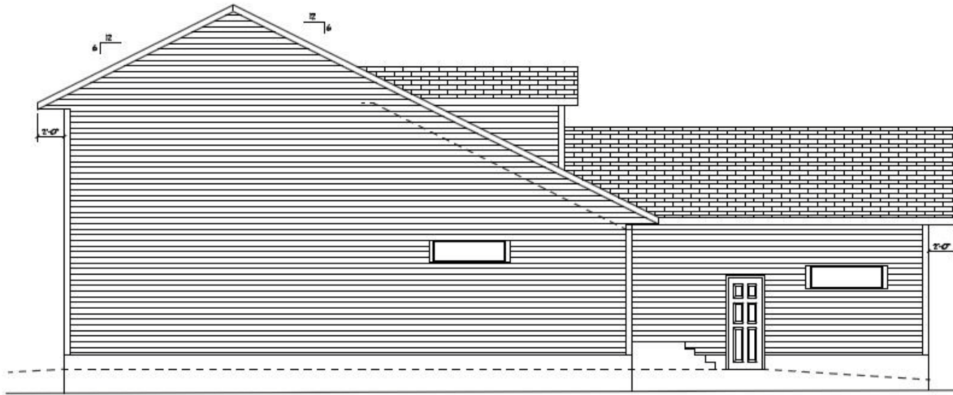
LEFT ELEVATION
